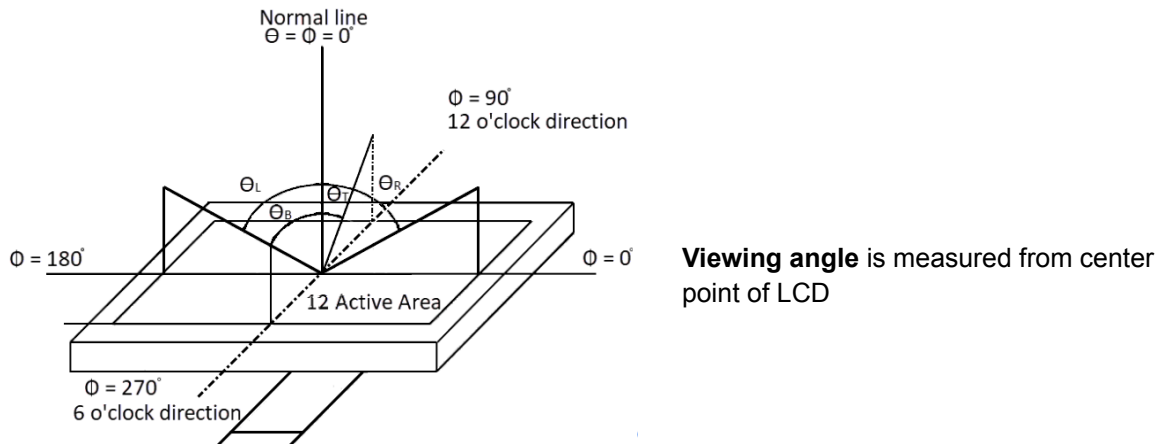
Figure 5: Viewing Angles
