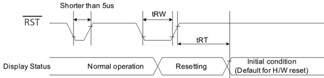
Figure 5: Reset Timing
